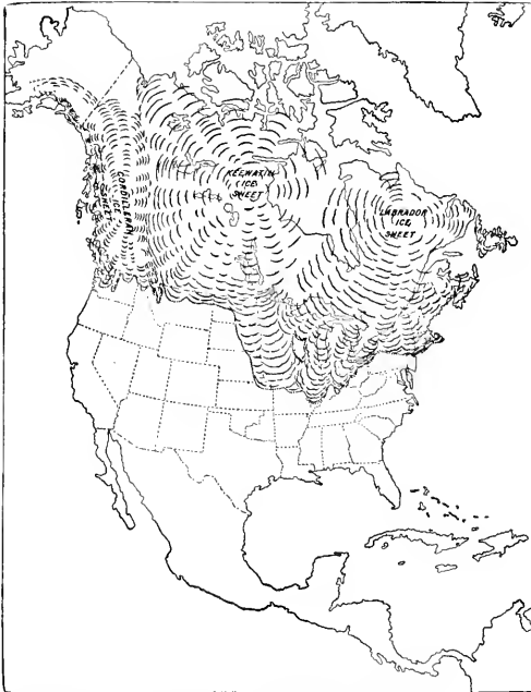
FIG. 19. Map showing maximum extent of ice sheets of Glacial period in North America. (U. S. Geol. Surv.)
